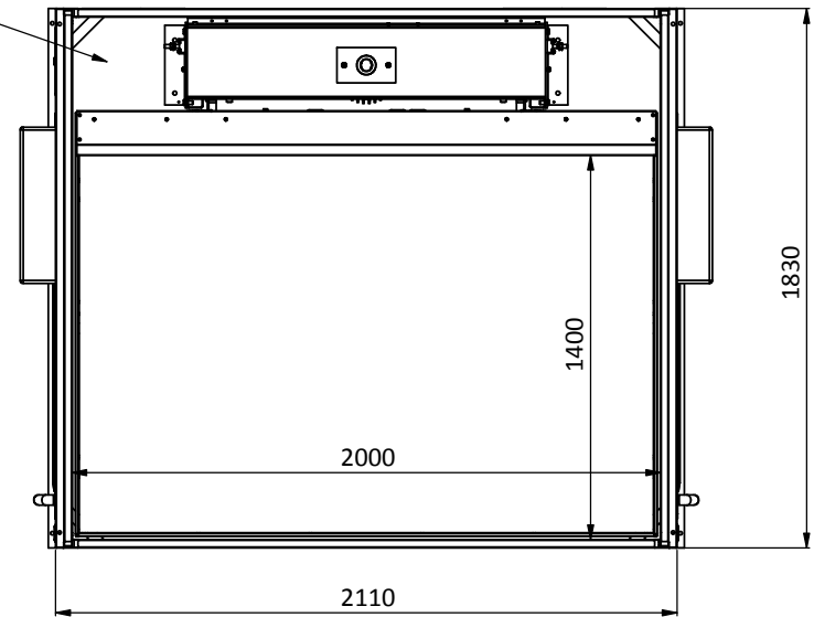
Overall dimensions
